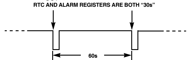
FIGURE 14. \overline{IRQ}/F_{OUT} WAVEFORM
